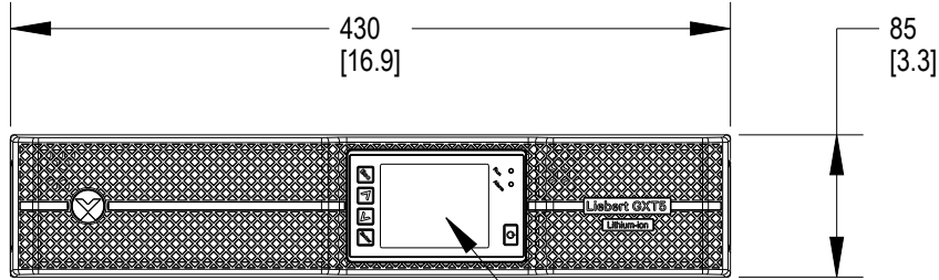
FRONT VIEW FOR DETAIL SEE DRAWING GXT5-DISPLAY
