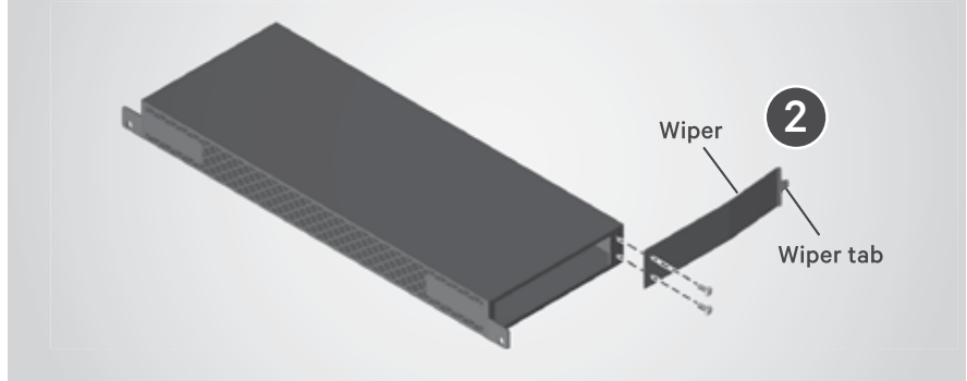
Geist SwitchAir Wiper Installation
